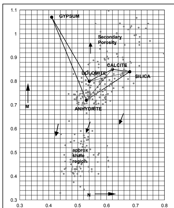
Fig. (5) M-N plot of Upper Bahariya Formation for Bassel-1x well.
