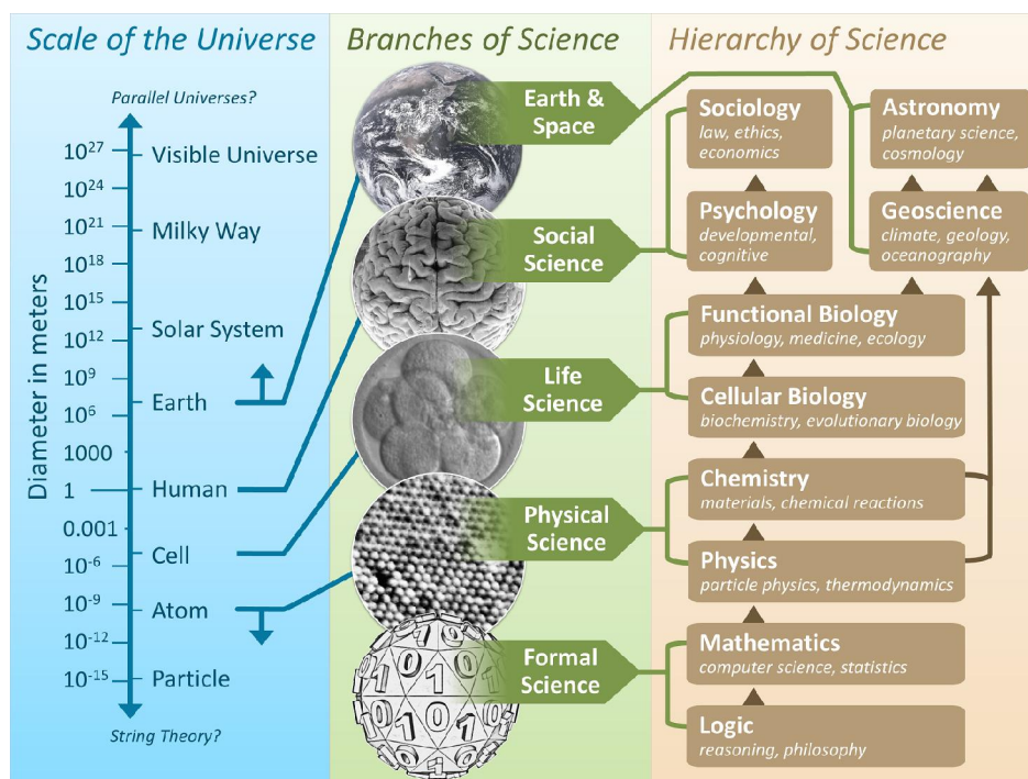
The scale of the universe mapped to the branches of science and the hierarchy of science.[6] Further information: Outline of science
